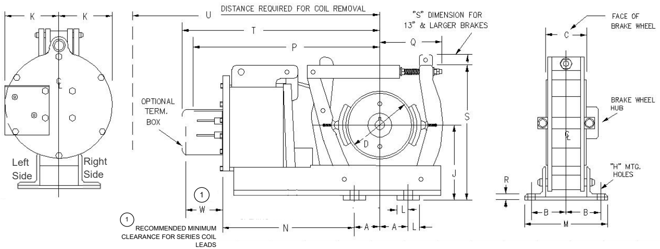
8-Inch Through 23-Inch Brakes
