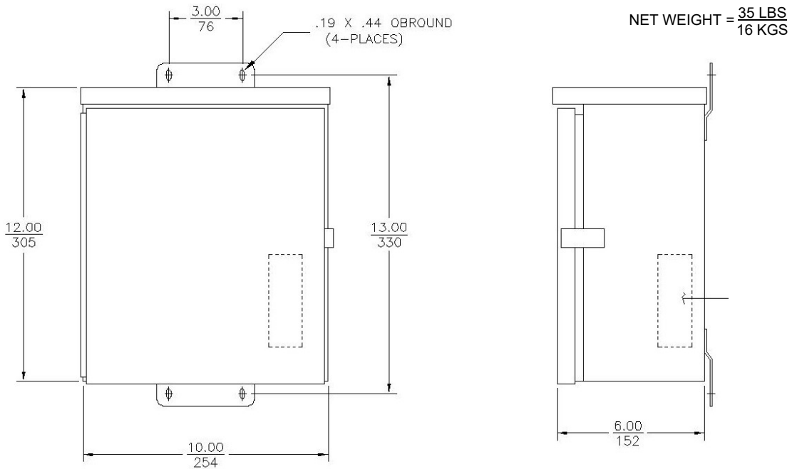
Types LC108, LC110, LC113, LC208, LC210
