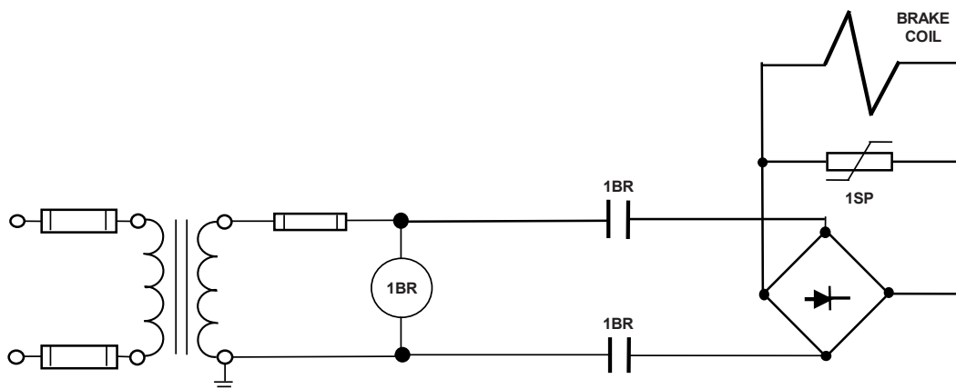
AC Rectifier Operated Brake, Type LC Brake Rectifier
