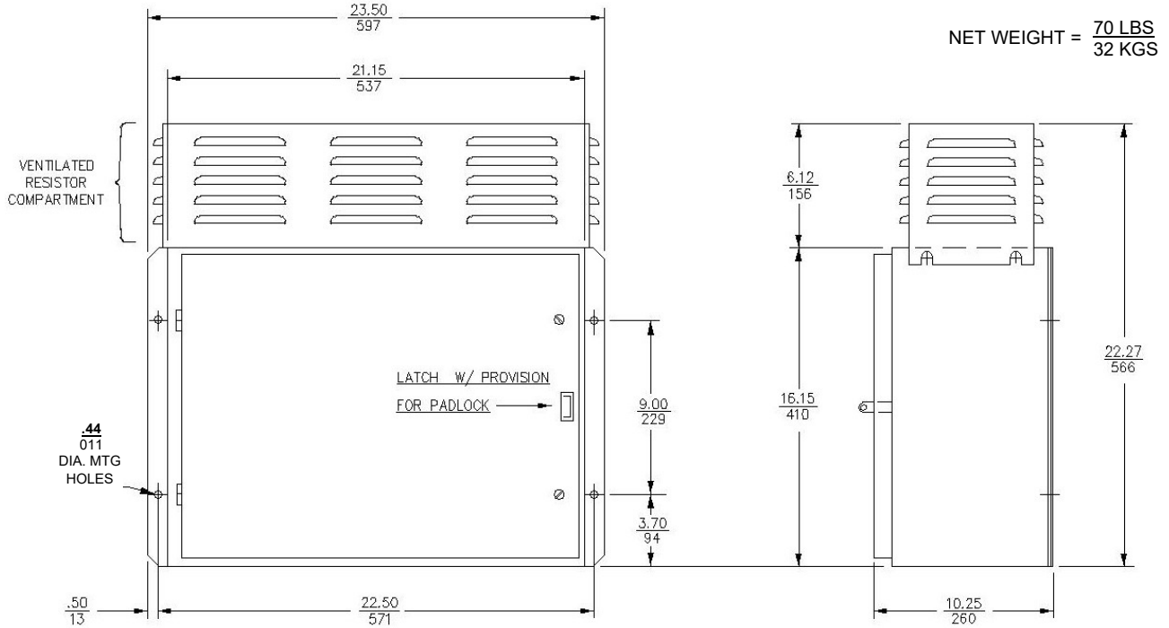
Types QW108 through QW130, QW208 through QW223
