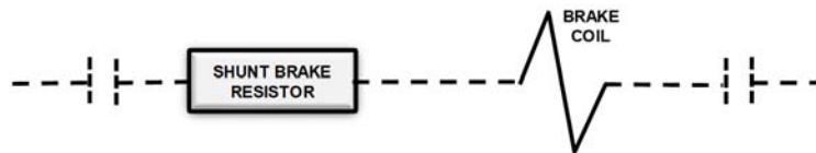
DC Standard Shunt Brake: (DC Travel Motions Only)
