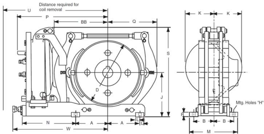
30-Inch Brakes
