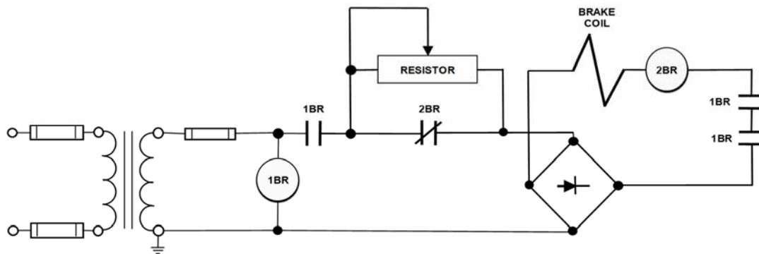
AC Rectifier Operated Brake, Type QW Brake Rectifier Controller
