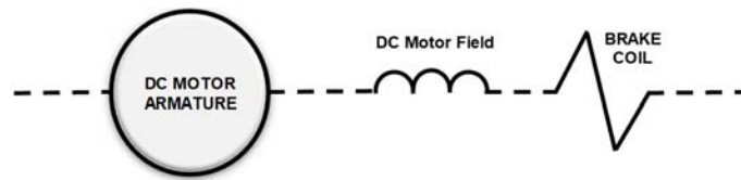
DC Series Brake: (DC Hoist or Travel Motions)
