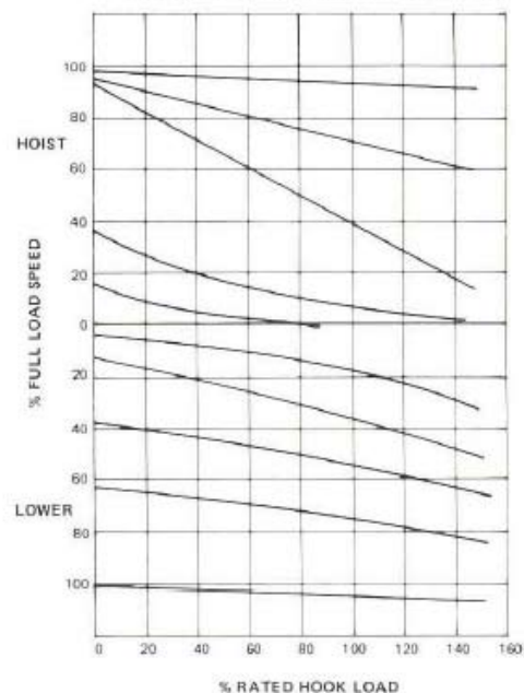
TYPICAL CRANE PERFORMANCE CURVES TYPE 4014 REVERSING CONTROL FOR USE WITH ELECTRIC LOAD BRAKE
